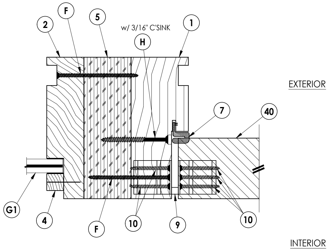
1 5 HORIZONTAL CROSS SECTION Inswing shown (Outswing similar)
