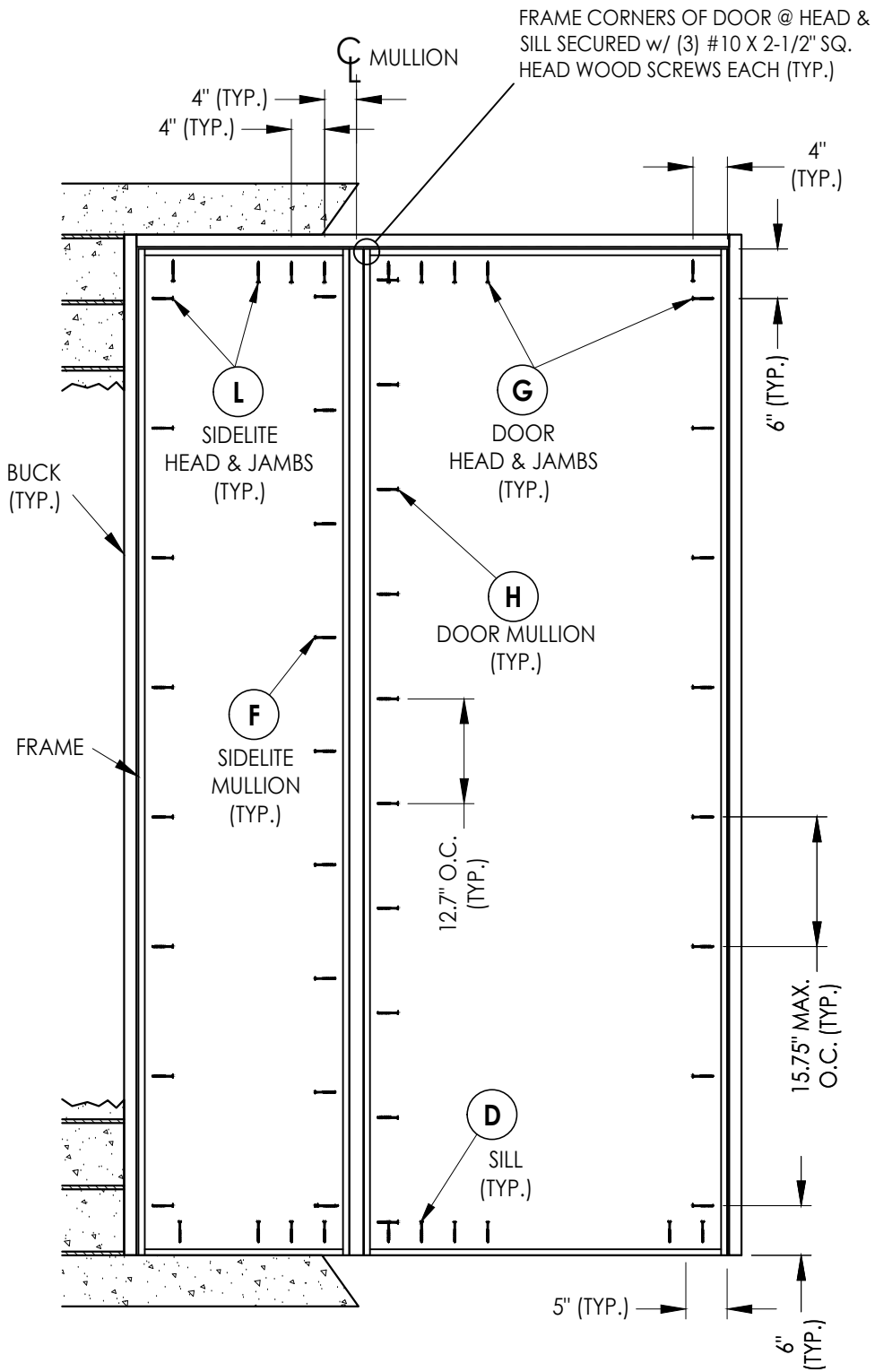
FRAME ANCHORING
