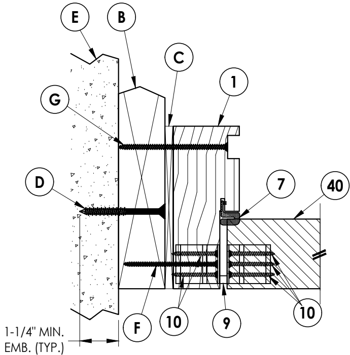
4 4 HORIZONTAL CROSS SECTION Inswing shown (Outswing similar)
