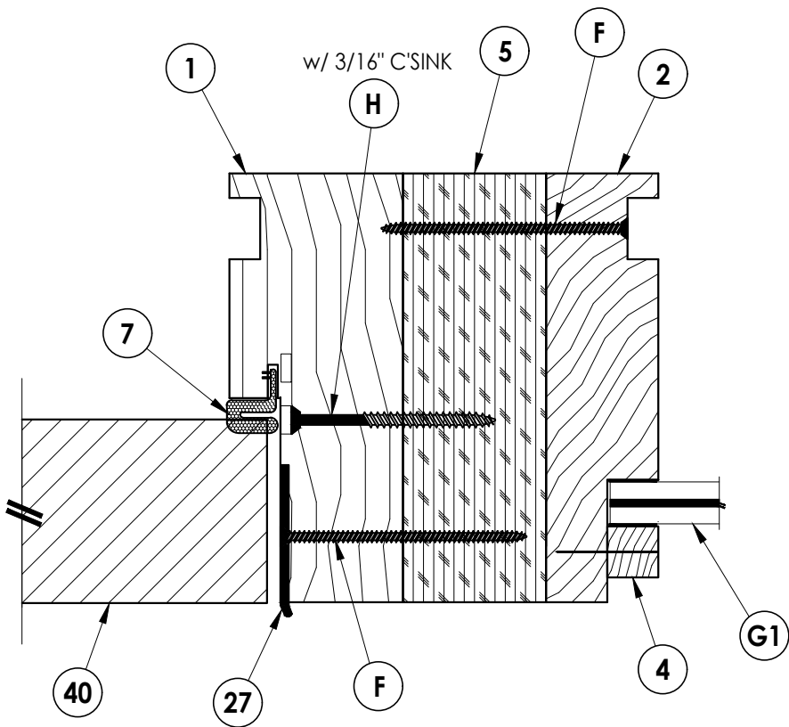
2 5 HORIZONTAL CROSS SECTION Inswing shown (Outswing similar)
