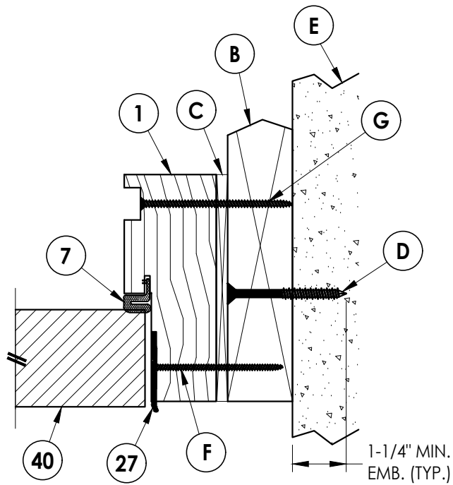
5 4 HORIZONTAL CROSS SECTION Inswing shown (Outswing similar)
