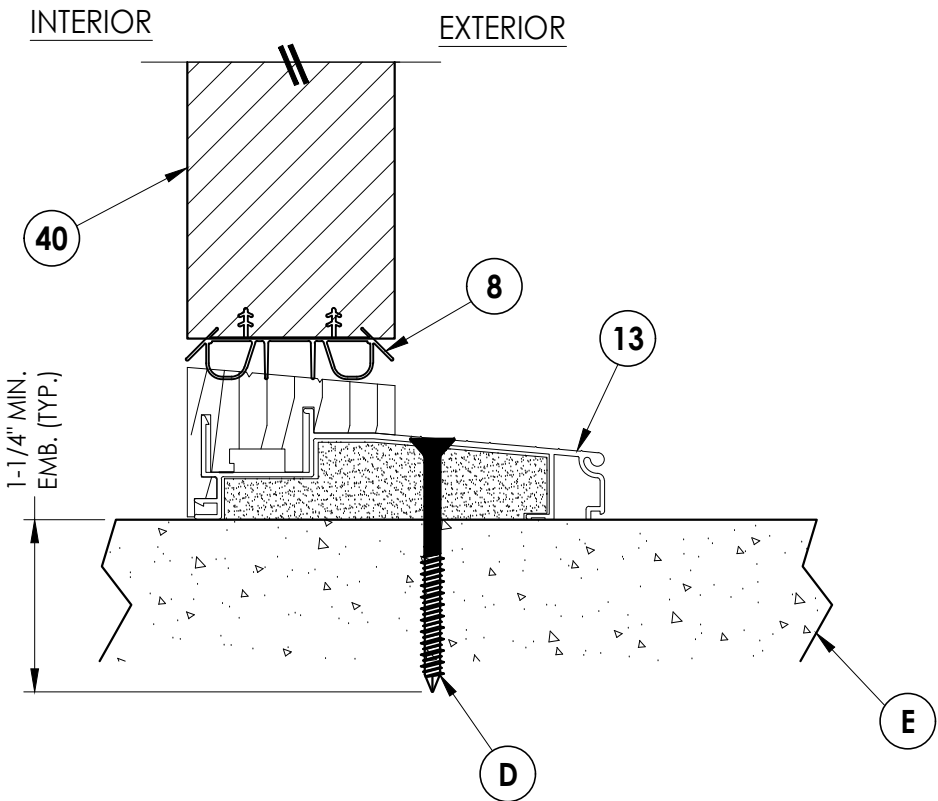
2 6 VERTICAL CROSS SECTION Inswing
