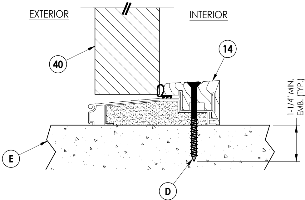
1 6 VERTICAL CROSS SECTION Outswing
