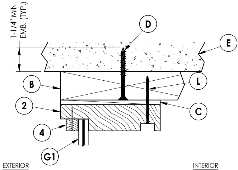
1 4 VERTICAL CROSS SECTION Inswing shown (Outswing similar)
