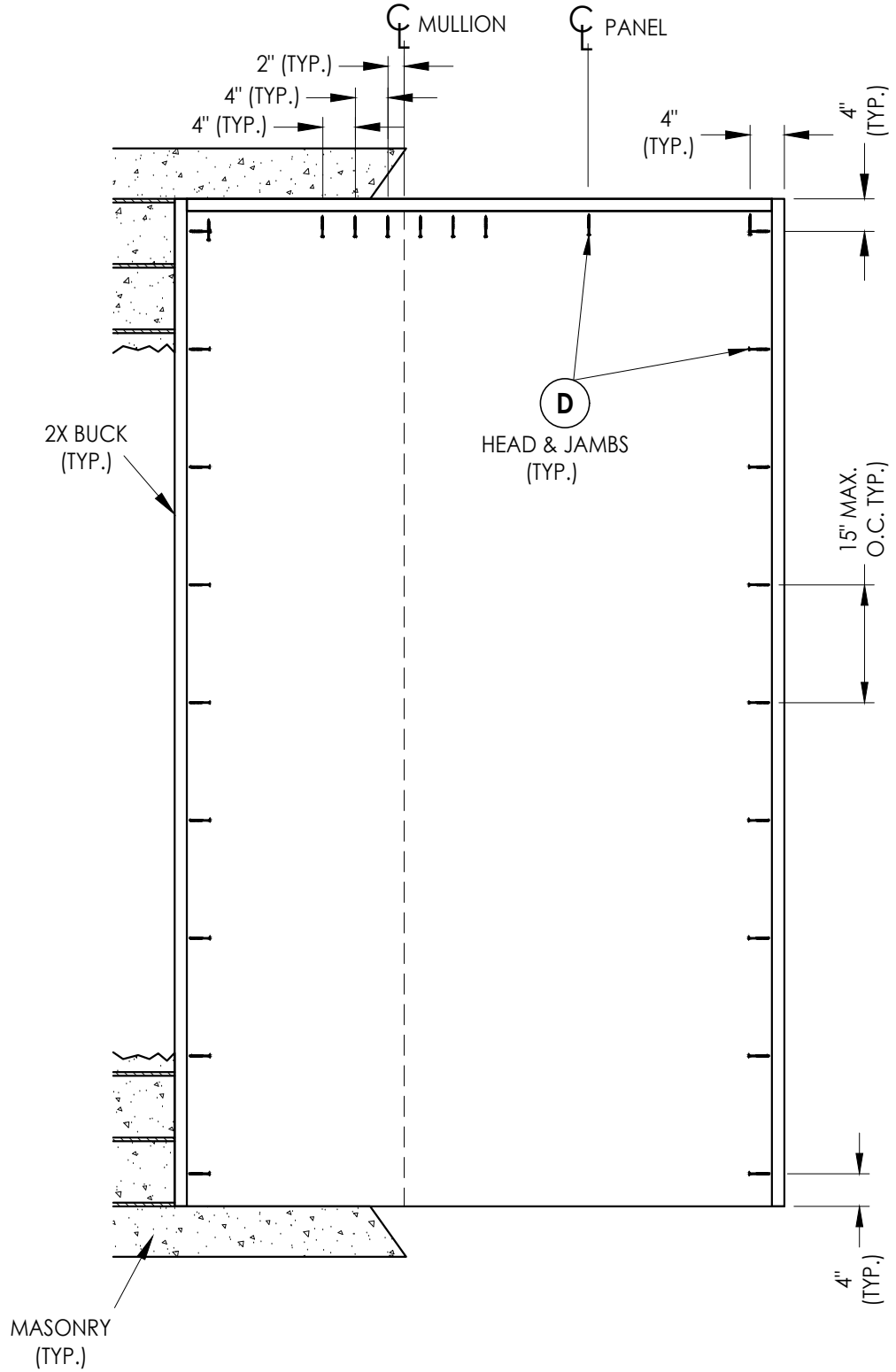
2X BUCK ANCHORING
