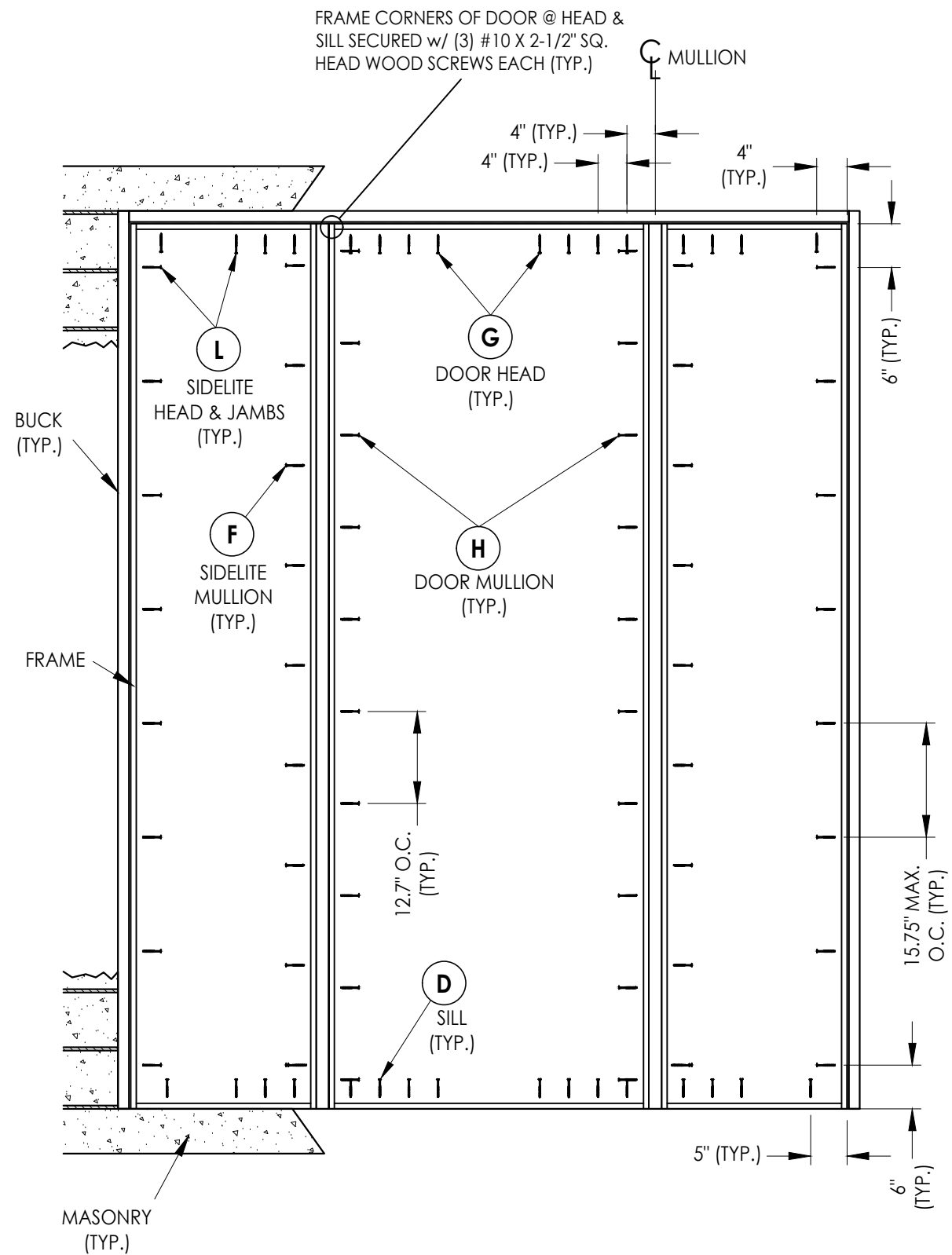
FRAME ANCHORING
