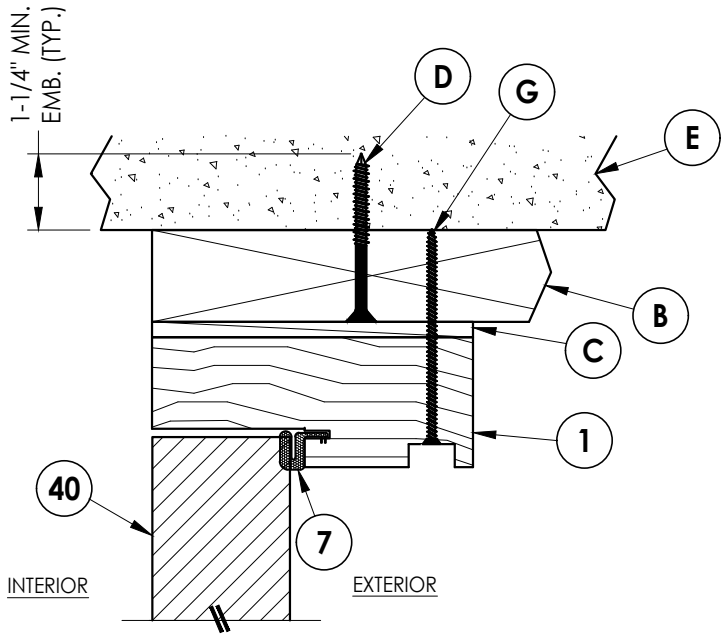
2 4 VERTICAL CROSS SECTION Inswing shown (Outswing similar)
