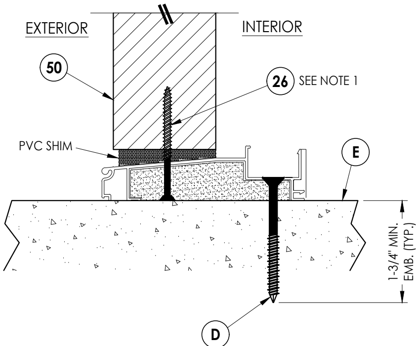
3 6 VERTICAL CROSS SECTION Inswing shown (Outswing similar)
