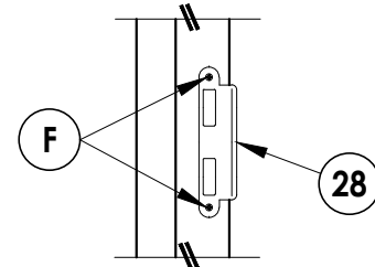
MULTIPOINT LOCK STRIKE DETAIL
